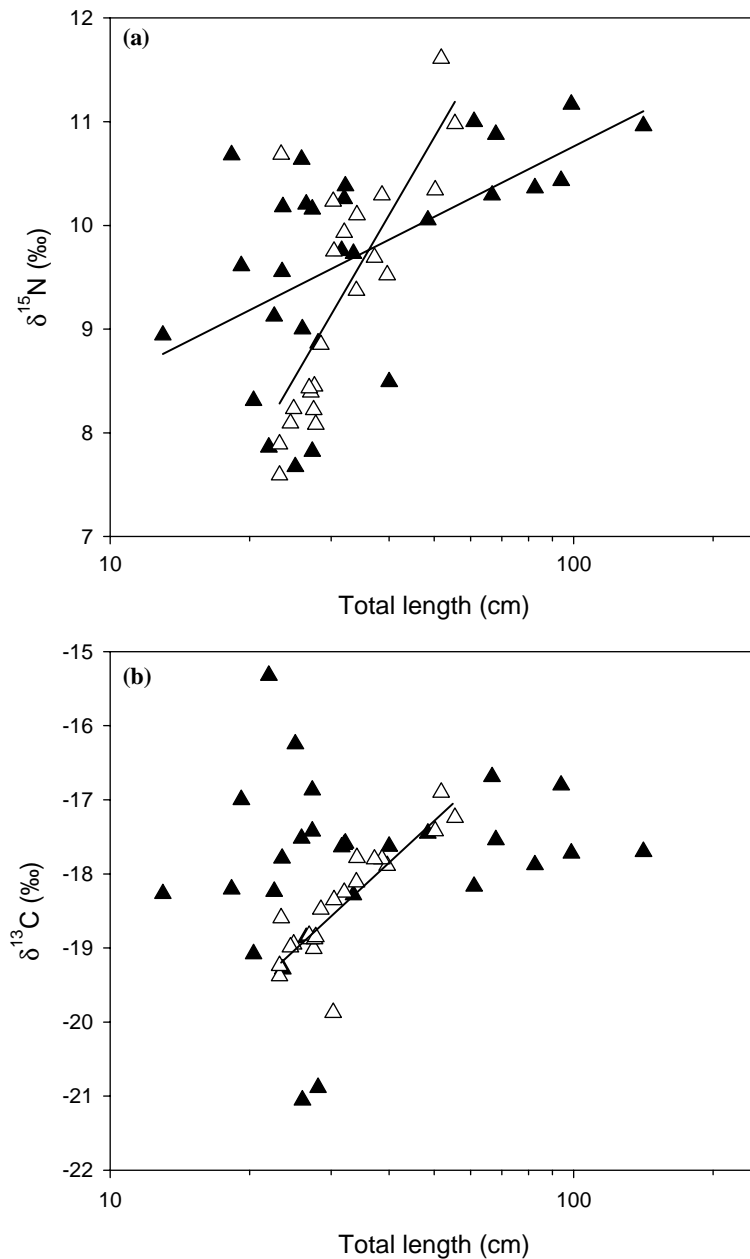
Figure 2. The relationships between \delta^{15}\text{N} (a) or \delta^{13}\text{C} (b) vs. total length (TL) for Lates macrophthalmus (open triangle) and L. niloticus (closed triangle).
