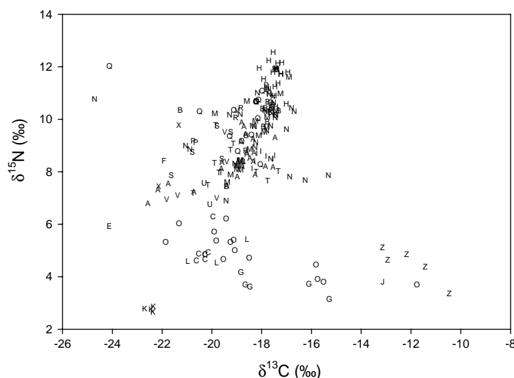
Figure 1. Stable isotope diagram for Lake Albert. The \delta^{13}\text{C} values on the x-axis represent potential carbon sources whereas \delta^{15}\text{N} on the y-axis generally can be interpreted as trophic level. Refer to Table 1 for the code key.
