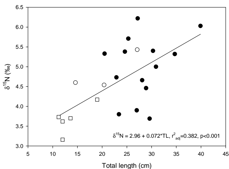
Figure 3. The regression of \delta^{15}\text{N} vs. total length for Oreochromis niloticus (closed circle), O. leucostictus (open circle) and Sarethorodon galilaeus (open square) grouped together to demonstrate possible size-dependent trends in tilapiine dietary patterns and habitat niches. No significant correlations were found within each tilapiine species.
