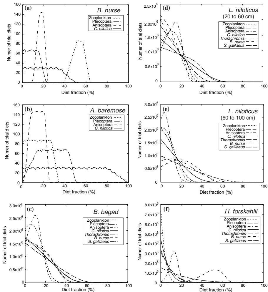
Figure 4. Results from the parameter search for 6 Lake Albert fish species. The graphs show the frequency of a given percentage contribution to the overall diet for each dietary item. B. nurse and H. forskahlii , which are known to have specialized diets, show clearly demarcated peaks for two dietary items that also coincide with literature stomach content data (Table 4). The other fish species, all opportunistic predators, demonstrate multiple overlaps indicating that there are a large number of possible dietary combinations for those species.
